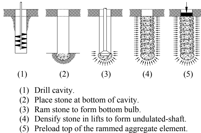
Figure 1: Construction Process
